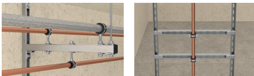
Time-saving installation of pipelines until 2" / 4 " with threaded rods and hanger bolts
